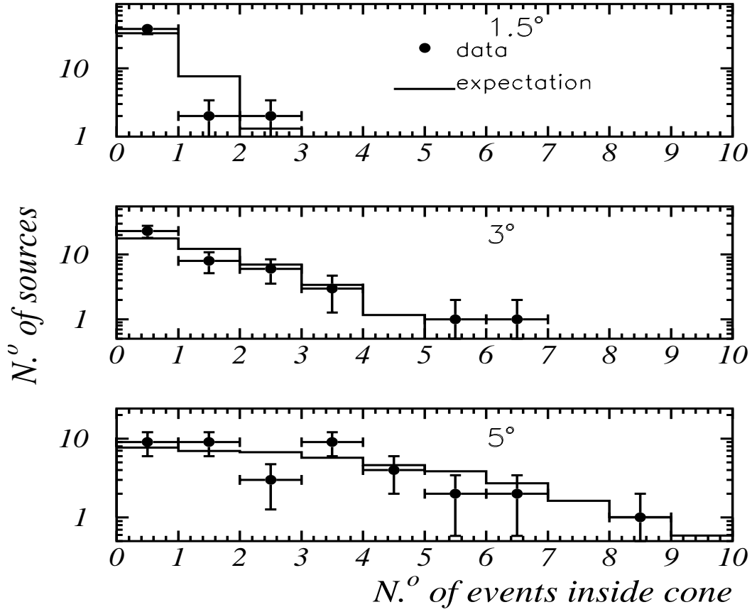
Fig. 11.— On the x axis there is the number of events falling in cones of half width 1.5^{\circ} , 3^{\circ} , 5^{\circ} (from top to bottom) around the direction of the 42 sources considered. The y axis depends on the total number of sources considered. Black circles: data. Solid line: simulation.
