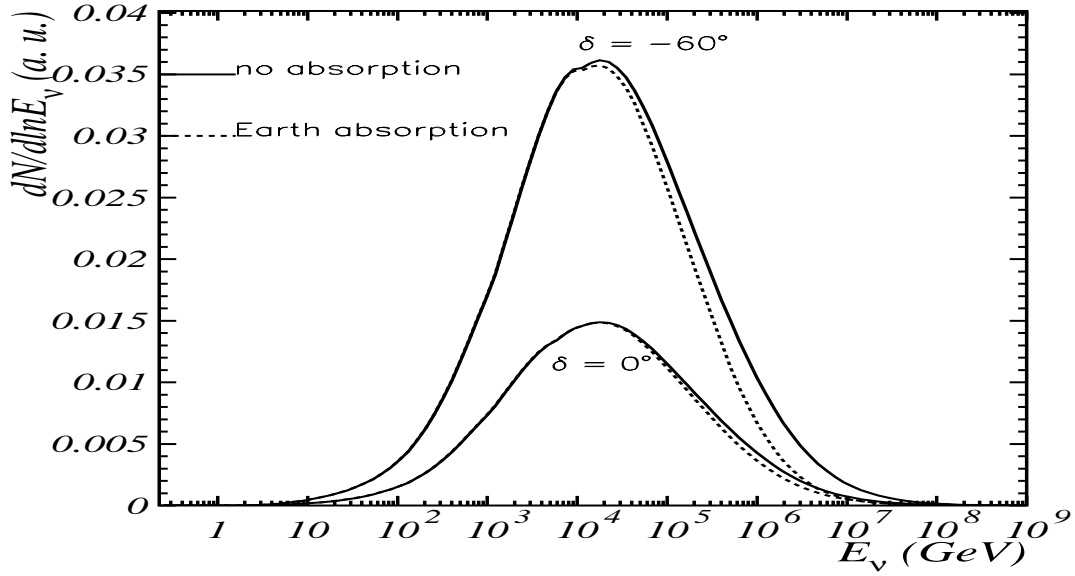
Fig. 6.— MACRO response curve, which is the differential rate of neutrinos which induce detectable muons as a function of the neutrino energy, for 2 sources at declinations -60^\circ and 0^\circ . Solid (dotted) lines do not (do) include Earth absorption. The normalization of the neutrino fluxes is arbitrary.
