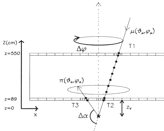
Fig. 2. Sketch of an event containing a down-going muon with direction (\vartheta_\mu, \varphi_\mu) producing an up-going pion with direction (\vartheta_\pi, \varphi_\pi) . The arrows indicate the direction of the particles, deduced from the timing information obtained from the scintillation counters ( T_1 , T_2 and T_3 ). The filled points correspond to the streamer tube hits. The zenith and azimuth emission angles \Delta\alpha , \Delta\varphi of the pion with respect to the muon direction are indicated.
