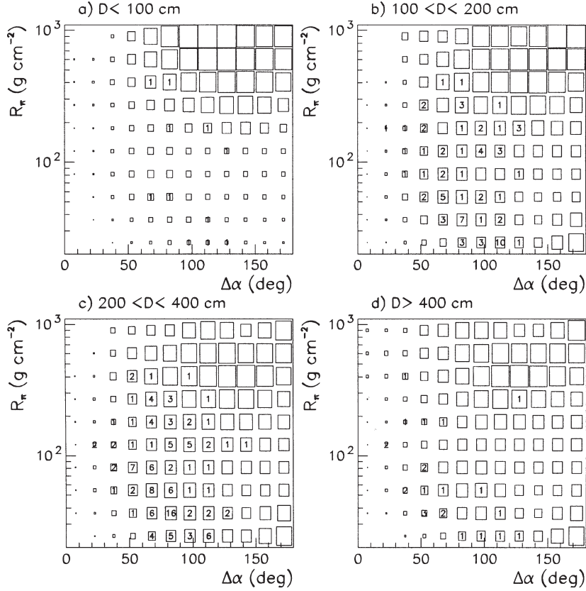
Fig. 7. Reconstruction efficiency AE in the (R_\pi, \Delta\alpha, D) parameter space, for 4 intervals of the distance D , 12 bins of \Delta\alpha and 10 bins of the measured range of the pion inside the detector R_\pi . The computed values of AE are proportional to the box area. For example, the upper row in (d) corresponds to values of (AE \cdot 100) equal to 1, 1, 3, 18, 29, 48, 52, 47, 40, 30, 48 and 76. In each cell the number of detected muon plus up-going pion events at the given (R_\pi, \Delta\alpha, D) values is indicated.
