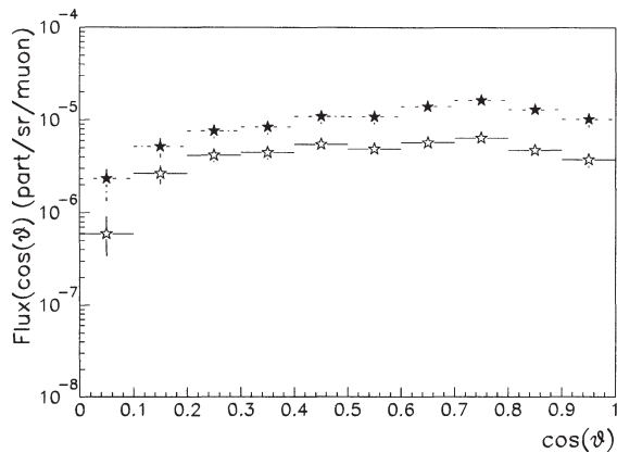
Fig. 9. Angular distribution of the charged particles emerging from the floor, \vartheta , relative to the vertical direction. The flux is normalized to the total number of detected single muons ( 12.2 \times 10^6 ). Open stars: uncorrected data. Full stars: corrected and detector-unfolded data for pions with scattering angles \Delta\alpha > 45^\circ . The pion energy threshold is around 100 MeV. Only statistical errors are shown.
