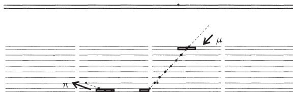
Fig. 1. On-line display of a typical muon interaction in the rock below the apparatus giving rise to an up-going charged particle. The rectangular boxes indicate scintillator counter hits and the points are streamer tube hits. The tracks are shown in the wire view of the streamer tubes. Only two supermodules are drawn.
