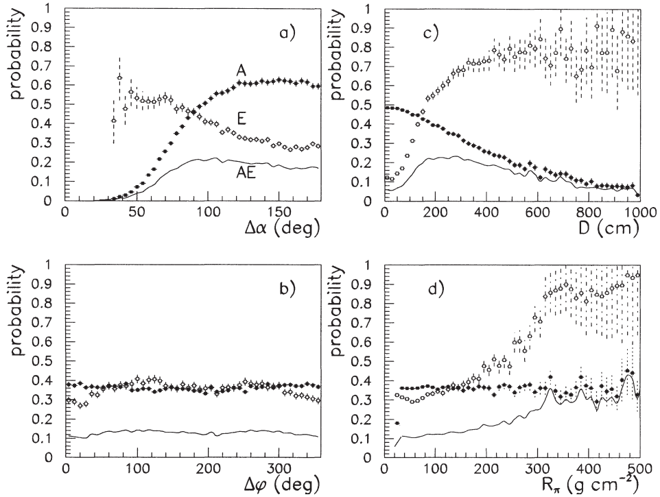
Fig. 6. Distribution of the probability A for events to be accepted, of the tracking efficiency E , and of the reconstruction efficiency AE versus (a) \Delta\alpha , (b) \Delta\phi , (c) D , and (d) R_\pi . Each quantity is averaged over the three remaining variables. Full points: A ; empty points: E ; solid curves: AE .
