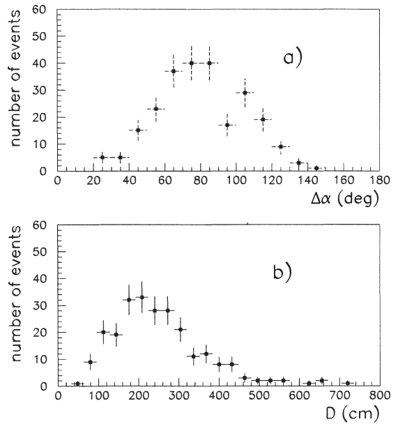
Fig. 5. (a) Measured distribution of the \pi - \mu scattering angle \Delta\alpha and (b) of the distance D between the down-going muon and the up-going pion at the z location of the center of the bottom layer of scintillation counters.
