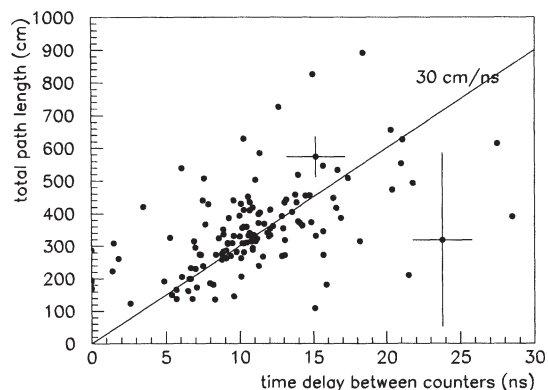
Fig. 3. Total path length (see text) versus time delay \Delta t = (T_3 - T_2) between scintillation counter hits in the bottom plane. Only the 168 events for which |z_v^w - z_v^s| < 50 cm are included. The large spread around the central line is due to the combined uncertainty in the total path length and timing reconstruction. As an example, error bars are drawn for two events. For three events, T_2 is missing and \Delta t = 0 .
