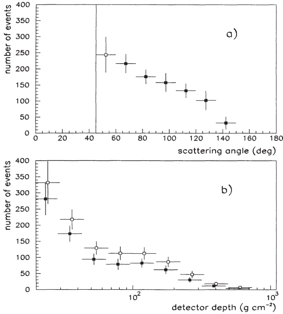
Fig. 8. (a) Detector-unfolded distribution of the zenith scattering angle \Delta\alpha of the pion with respect to the muon direction for \Delta\alpha > 45^\circ . (b) Detector-unfolded distribution of the up-going pion range inside the detector. Open points: pions with \Delta\alpha > 45^\circ ; full points: pions with \Delta\alpha > 60^\circ (b). Only statistical errors are shown. The number of events corresponds to 1.55y of data taking.
