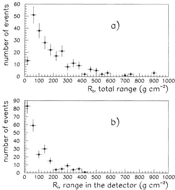
Fig. 4. (a) Distribution of the reconstructed total range R_t of the up-going particles for which |z_v^w - z_v^s| < 50 cm. Events with a poorly reconstructed vertex are excluded from this distribution because of the large uncertainty in R_t for these events. (b) Distribution of the grammage traversed in the detector, R_i , for all the 243 up-going particles in the final data set.
