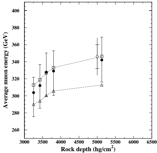
Fig. 9. Average single muon energy measured by the MACRO TRD (black circles) versus standard rock depth. The open symbols connected by dashed lines are the predictions of a HEMAS-based Monte Carlo for the “Light” (squares) and “Heavy” (triangles) composition models. The result reported by the NUSEX experiment is shown by the diamond (the extensions of the error bar represents the systematic uncertainty added in quadrature to the statistical error [4]).
