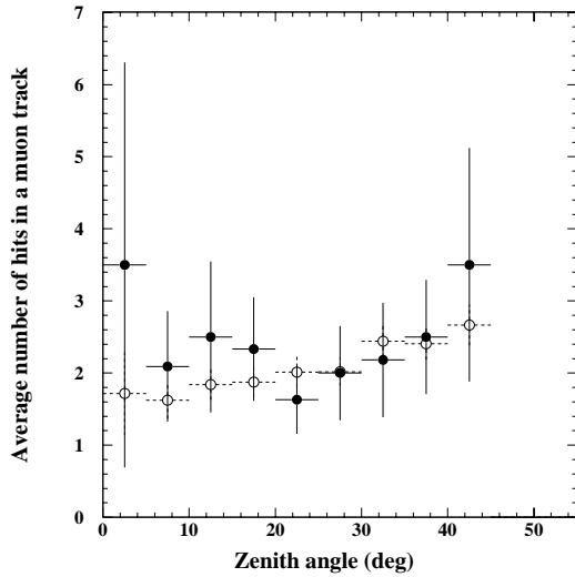
Fig. 4. Average number of hits versus zenith angle for muons crossing the TRD and stopping in the lower MACRO detector. Black circles: TRD data; open circles: Monte Carlo simulation. Only statistical errors are shown.
