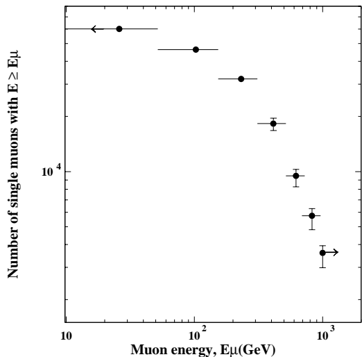
Fig. 6. Integral energy distribution of single muons with zenith angle \leq 45^\circ measured with the TRD. The spectrum was obtained by unfolding the hit distribution shown in Fig. 3.
