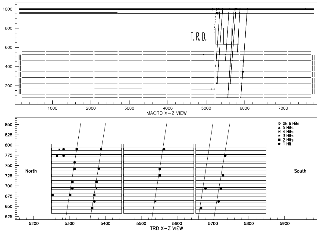
Fig. 2. Display of a multiple muon event crossing MACRO and the TRD. The upper part of figure shows the whole MACRO detector in the view orthogonal to the streamer tubes, while in the lower part only the TRD in the view orthogonal to proportional tubes is shown. The number of hits produced in the TRD are shown by different symbols. While the second muon from the right has E_\mu approximately 200 GeV, the other muons have energies of roughly 500 GeV.
