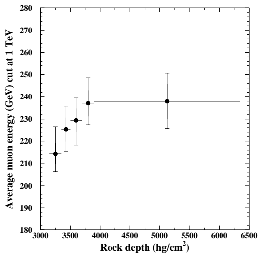
Fig. 7. Average single muon energy, computed with a cut at 1 TeV, versus the standard rock depth.
