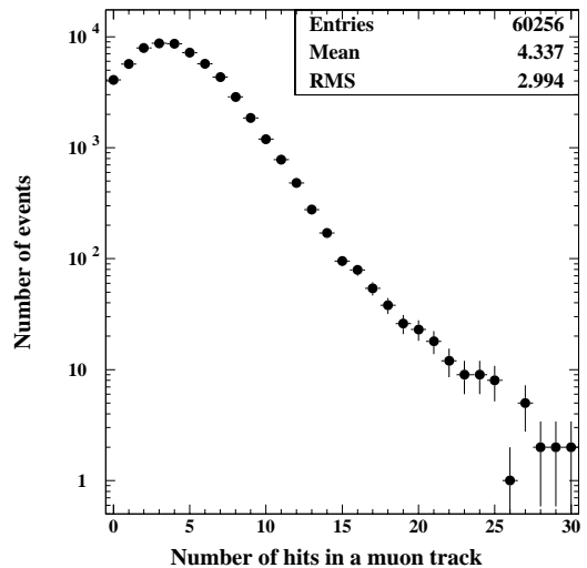
Fig. 3. Hit distribution for single muon tracks crossing the 10 TRD planes with zenith angles less than 45^\circ . Only statistical errors are shown.
