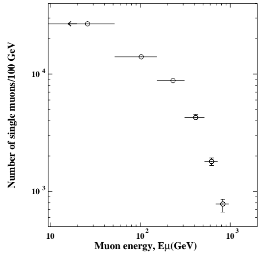
Fig. 5. Differential energy distribution of single muons with zenith angle \leq 45^\circ measured with the TRD. The spectrum was obtained by unfolding the hit distribution shown in Fig. 3.
